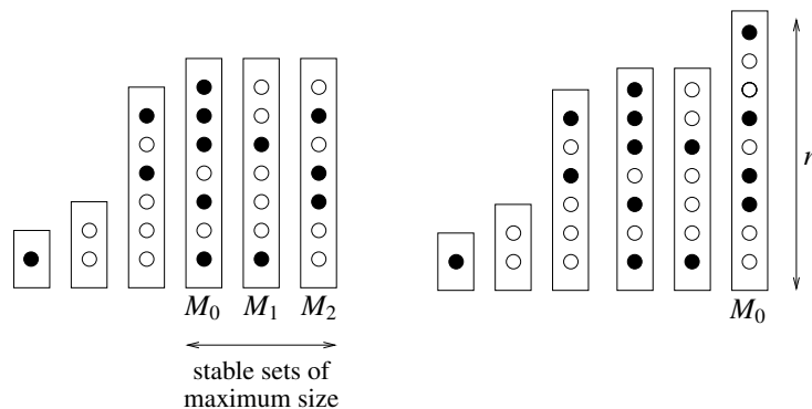
Figure 11. Left: 6-partite complete graph with three maximum independent sets. Right: 6-partite complete graph with a unique maximum independent set.
