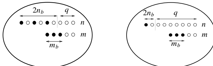
Figure 9. Two examples of positions satisfying f(\Phi) < 0 .
