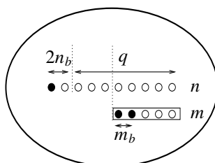
Figure 10. A position satisfying f(\Phi) \geq 0 .
