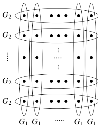
Figure 3. The Cartesian product of two graphs G_1 and G_2 .
