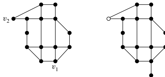
Figure 4. Reduction to a Hamiltonian path.
