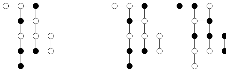
Figure 2. Left: play on a grid graph G . Right: play on complementary copies of G .
