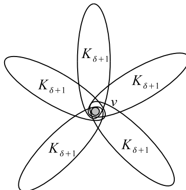
Figure 12. The graph S_k(K_{d+1}) .
