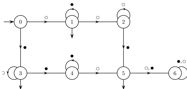
Figure 6. Automaton for 1-reducible paths.
