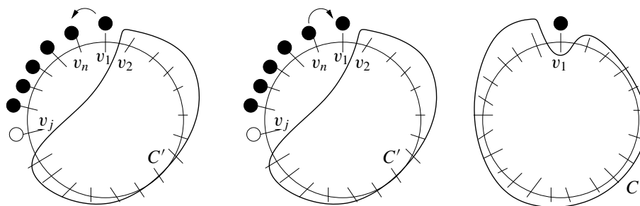
Figure 7. Possible fates for v_1 . Left: v_1 captures v_2 . Middle: v_1 is captured by v_2 . Right: v_1 is not involved in the move.
