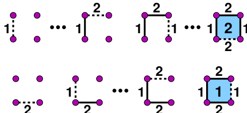
Figure 4. Behavior of a nonend box under Player 1's strategy, depending on who takes the first box edge. Top: Player 1 starts. Bottom: Player 2 starts. Nonimmediate responses are denoted by \dots .
