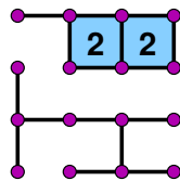
Figure 1. In the middle of a typical Dots-and-Boxes game. Based on [Berlekamp et al. 2003, Figure 1].
