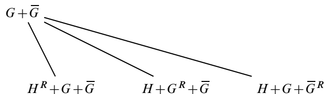
Figure 4. Right's possible opening moves in H + G + \bar{G} .
