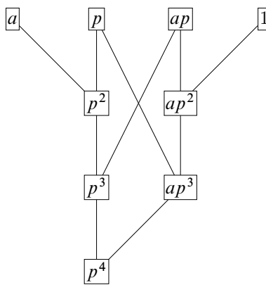
Figure 6. The partially ordered set of \mathcal{Q}(\text{cl}(\downarrow)) .
