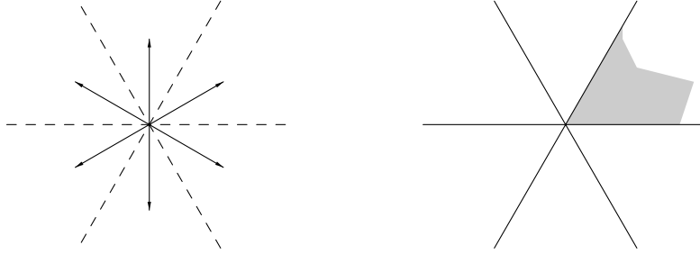
Figure 2. Left: Root system for A_2 . Right: A chamber for A_2 .
