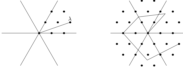
Figure 4. Left: Straight line path from 0 to \lambda . Right: A path in \mathcal{P}\pi_\lambda .
