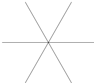
Figure 1. Hyperplane arrangement for A_2 .
