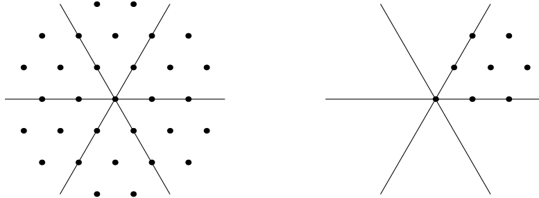
Figure 3. Left: The lattice of integral weights. Right: The cone of dominant integral weights.
