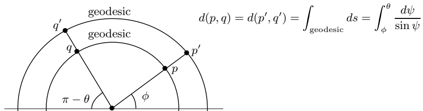
Figure 24. The formula for d(p, q) .
