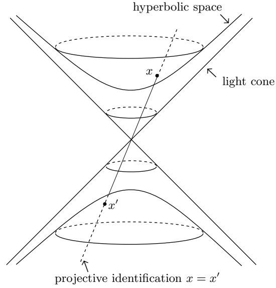
Figure 1. Minkowski space.
