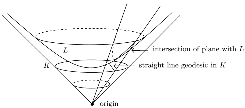
Figure 16. Geodesics in K and L .
