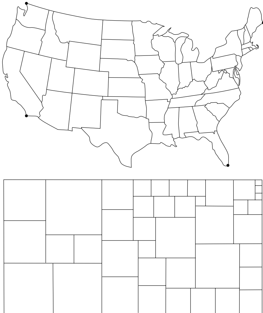
Figure 39. Combinatorial Riemann mapping.
